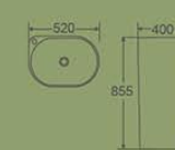
10019PW Pedestal Basin 520×400×855mm Fixing To Wall With Back Vitreous china
