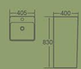
10005PW Pedestal Basin 405×400×830mm Fixing To Wall With Back Vitreous china
