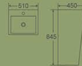
10001PW Pedestal Basin 510×450×845mm Fixing To Wall With Back Vitreous china
