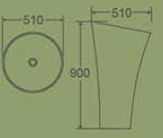
10044PW Pedestal Basin 510×510×900mm Fixing To Wall With Back Vitreous china
