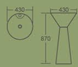
10028PW Pedestal Basin 430×430×870mm Fixing To Wall With Back Vitreous china
