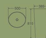
10015PW Pedestal Basin 500×385×815mm Fixing To Wall With Back Vitreous china
