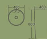
10009PW Pedestal Basin 460×460×860mm Fixing To Wall With Back Vitreous china
