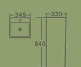
10003PW Pedestal Basin 345×330×840mm Fixing To Wall With Back Vitreous china
