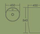
10043PW Pedestal Basin 450×450×840mm Fixing To Wall With Back Vitreous china
