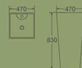
10004PW Pedestal Basin 470×470×830mm Fixing To Wall With Back Vitreous china
