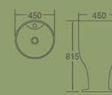
10042PW Pedestal Basin 450×450×815mm Fixing To Wall With Back Vitreous china
