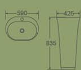
10020PW Pedestal Basin 590×425×835mm Fixing To Wall With Back Vitreous china
