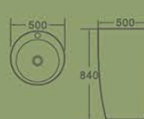
10014PW Pedestal Basin 500×500×840mm Fixing To Wall With Back Vitreous china
