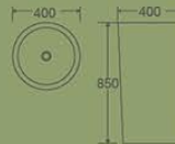
10011PW Pedestal Basin 400×400×850mm Fixing To Wall With Back Vitreous china
