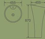
10027PW Pedestal Basin 455×455×870mm Fixing To Wall With Back Vitreous china
