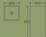
10008PW Pedestal Basin 400×400×850mm Fixing To Wall With Back Vitreous china
