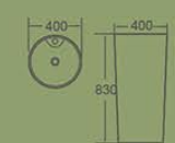
10010PW Pedestal Basin 400×400×830mm Fixing To Wall With Back Vitreous china
