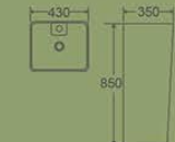
10007PW Pedestal Basin 430×350×850mm Fixing To Wall With Back Vitreous china
