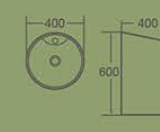
10013PW Pedestal Basin 400×400×600mm Fixing To Wall With Back Vitreous china
