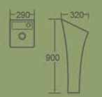
10029PW Pedestal Basin 290×320×900mm Fixing To Wall With Back Vitreous china
