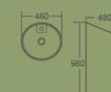
10012PW Pedestal Basin 460×480×960mm Fixing To Wall With Back Vitreous china
