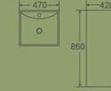
10006PW Pedestal Basin 470×420×860mm Fixing To Wall With Back Vitreous china
