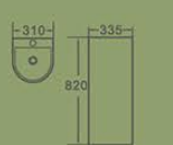
10017PW Pedestal Basin 310×335×820mm Fixing To Wall With Back Vitreous china
